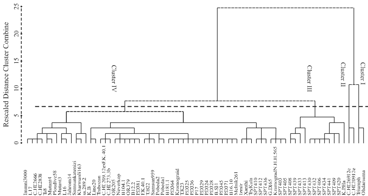
Figure 1 - UPGMA clustering of oriental tobacco genotypes based on squared Euclidean distances by using agro-morphological traits
