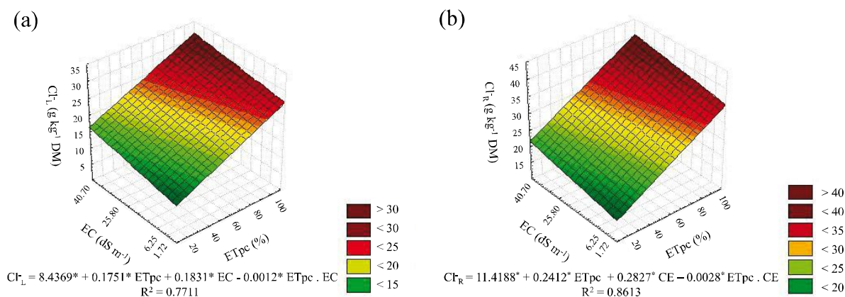
Figure 3 - Response surface for the Cl - ion content in the leaves (a) and roots (b) of young coconut plants for combinations of different levels of water deficit (% ETpc) and soil salinity (EC) at 120 DAT 1
