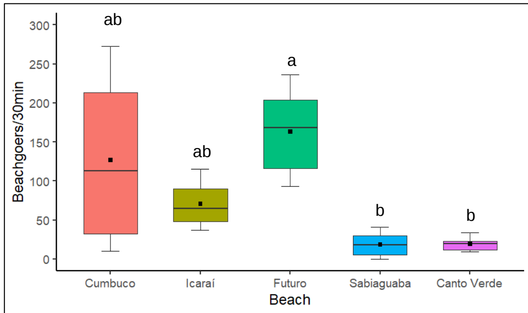
Figure 3 – Number of beachgoers observed for 30 minutes on the beaches of Cumbuco, Icaraí, Futuro, Sabiaguaba and Canto Verde. Black dot = mean, vertical bars = standard error. Different letters above the bars (standard error) indicate significant differences
