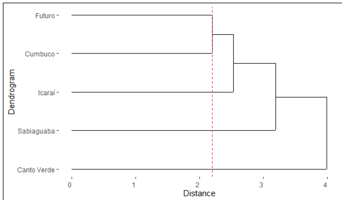
Figure 5 – Cluster analysis of urban intervention indicators (Gonzales et al. , 2014) and morphological indicators (grain size, beach slope and beach extension) of the beaches of Cumbuco, Icarai, Futuro, Sabiaguaba and Canto Verde
