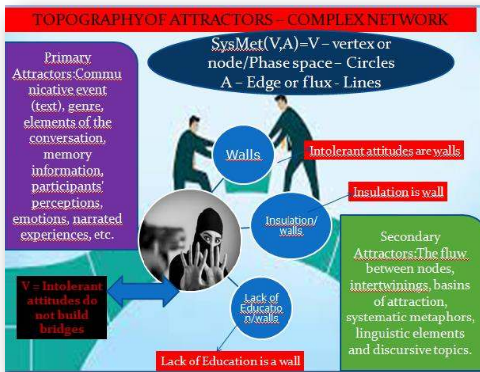
Figure 4 — Topology of attractors
