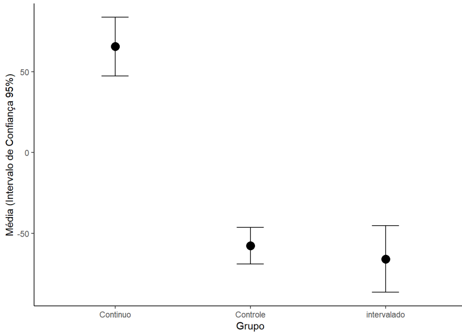
Gráfico 3: Comparison between groups regarding post-protocol MIP values
