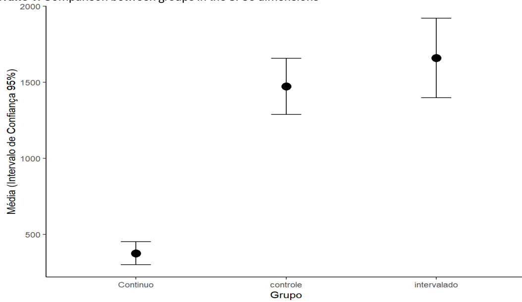
Grafic 1: Comparison between groups in the SF36 dimensions
