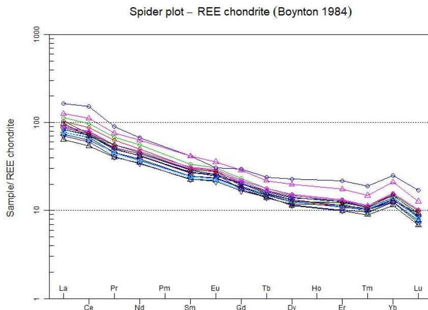
Figure 8A - the rare earth elements in mafic and neutral rocks in the study area based on the REE chondrite data
