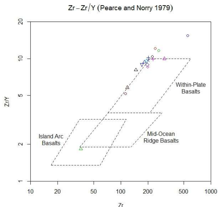
Figure 12 - The tectonic position of the rocks in the study area
