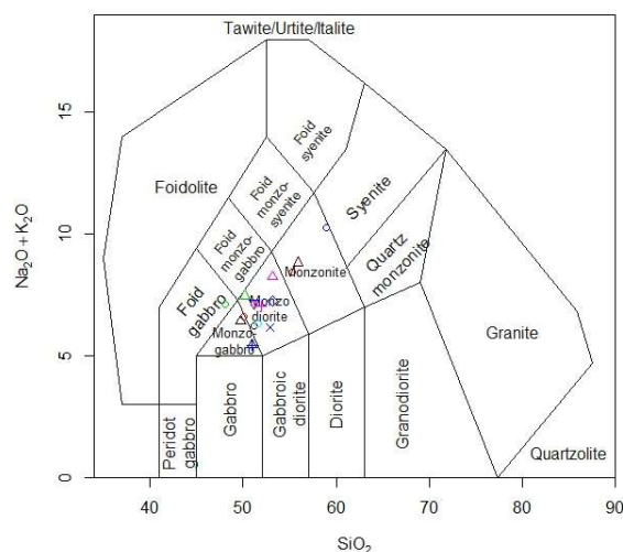
Figure 5 - Middlemost classification
