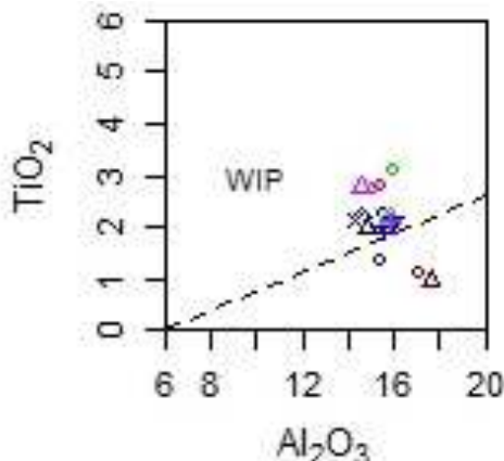
Figure 10 - The diagram of the tectonic position of the rocks in the study area
