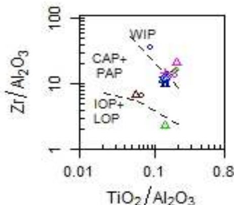
Figure 9 - The diagram of the tectonic position of the rocks in the study area
