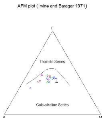
Figure 4 - Determining the calc-alkaline and tholeiitic series (Irvin and Barager, 1971)
