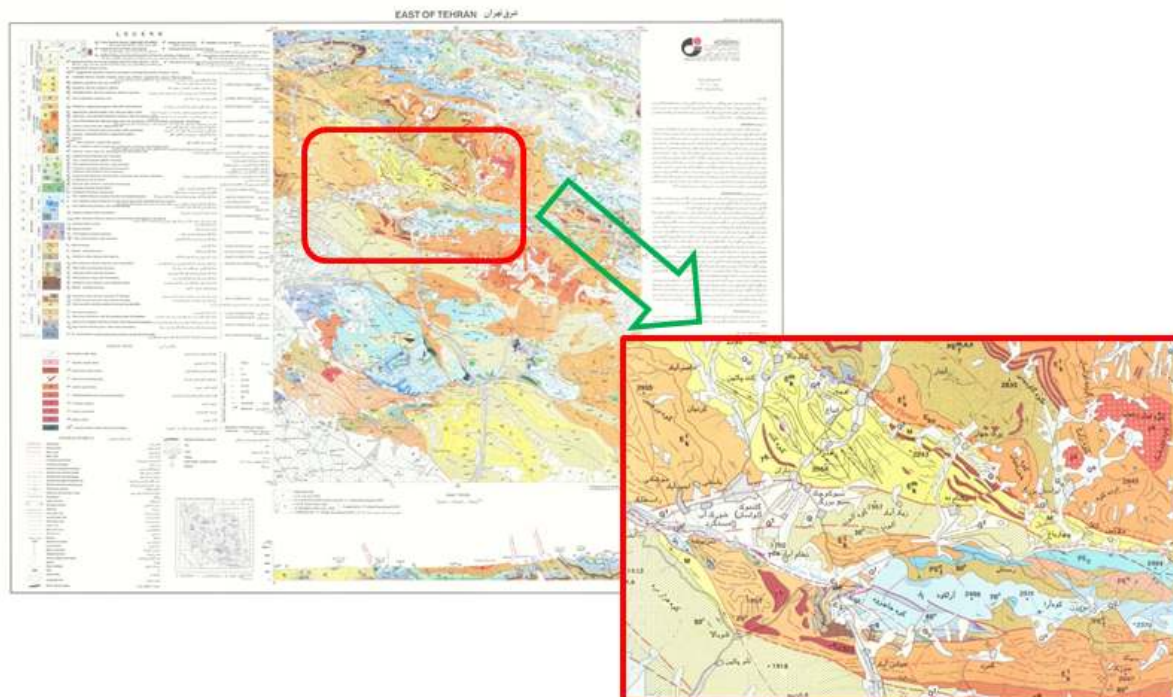
Figure 1 - The geological position of the study section
