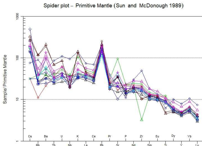
Figure 8B - Based on the primitive mantle
