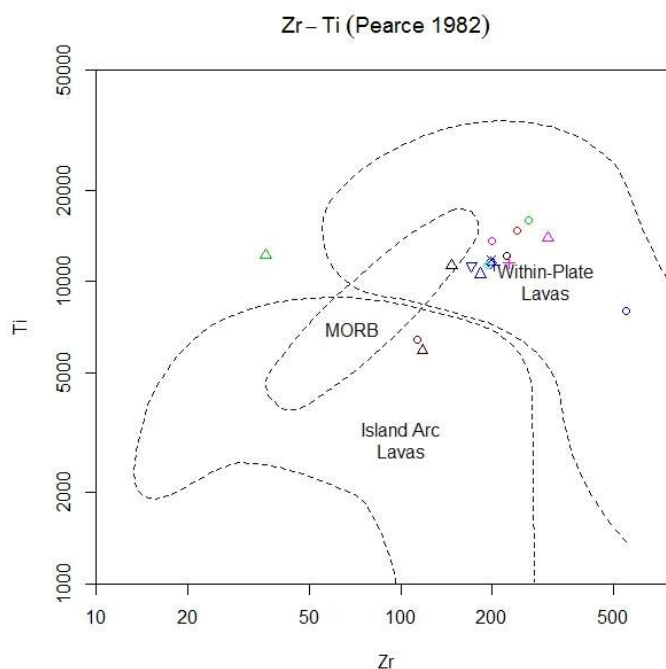
Figure 13 - The diagram of the tectonic position of the rocks in the region for the separation of island arc basalts, mid-ocean basalts, and within-plate basalts
