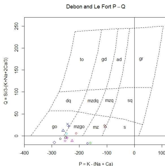
Figure 7 - The classification of the sills in the study area based on the accessory elements
