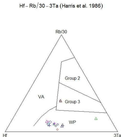
Figure 14 - The tectonic position of the sills in the region
