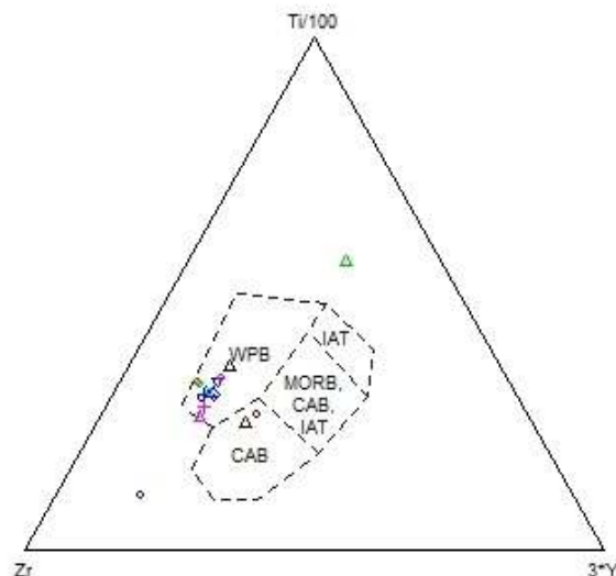
Figure 11 - The ternary diagram of the tectonic position of basalts for the differentiation of calc-alkaline, diagonal, island arc, and within-plate basalts
