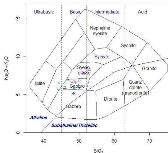
Figure 6 - The classification of the rocks in the study area
