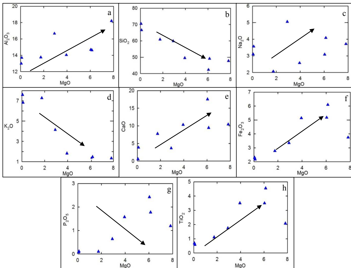
Figure 5 - Trends of Oxides of Main Elements vs. MgO
