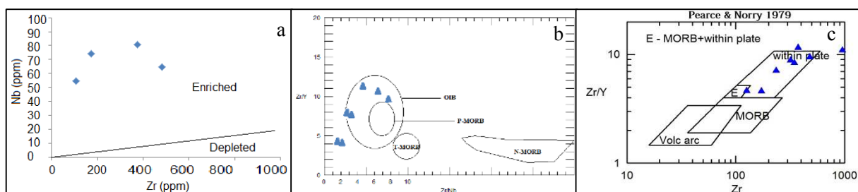
Figure 7 – a: Nb vs. Zr diagram (Abu-Hamattah et al. 2005) b: Zr / Nb vs. Zr / Y The samples studied are in the OIB range c: Pearce & Norry, 1979
