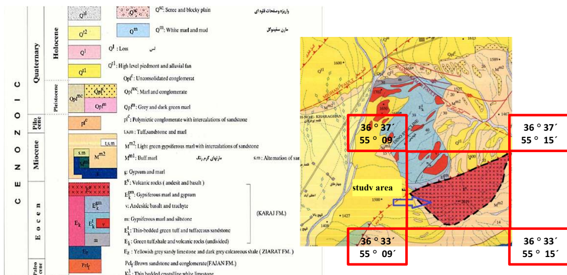
Figure 2 - Location of Siah Kooh region on a map of 1: 100000 Khosh Yeylagh map (Black Sea and 2004).
