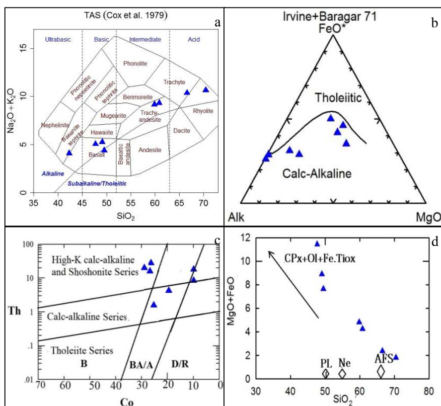
Figure 4: Diagram of \text{Na}_2\text{O} + \text{K}_2\text{O} vs. \text{SiO}_2 (Cox et al., 1979) B- Irvine and Baragar magmatic series diagrams, (1971) c. Tholeiitic and calc-alkaline ranges and location of samples in the region. Basalt: B, Basalt-Andesite: BA / A and Dacite and Rhyolite: D / R D - Graph of changes in total elemental elements ( \text{FeO} + \text{MgO} relative to \text{SiO}_2 Schrader 2001) for volcanic rocks in the region.
