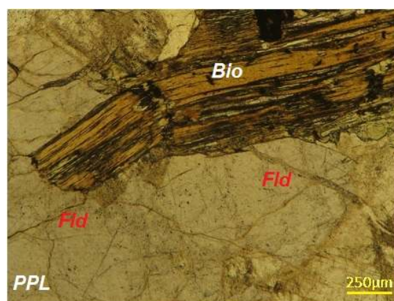
Figure 7 - Signs of bending and fracture are apparent in biotites due to tectonic pressure.
