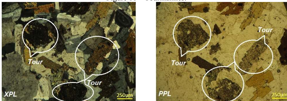
Figure 11 – Tourmalines.
