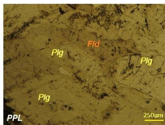
Figure 3 - Regular and oscillatory zoning in the plagioclase.
