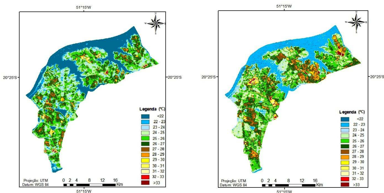
Figure 5 – Classified image of the estimated Surface Temperature for (a) 13/May/2000 and (b) 10/April/2011
