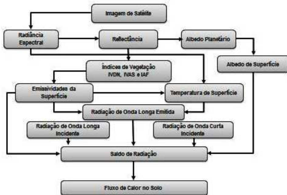
Figure 2 – Diagram of the SEBAL algorithm steps used in the study.
