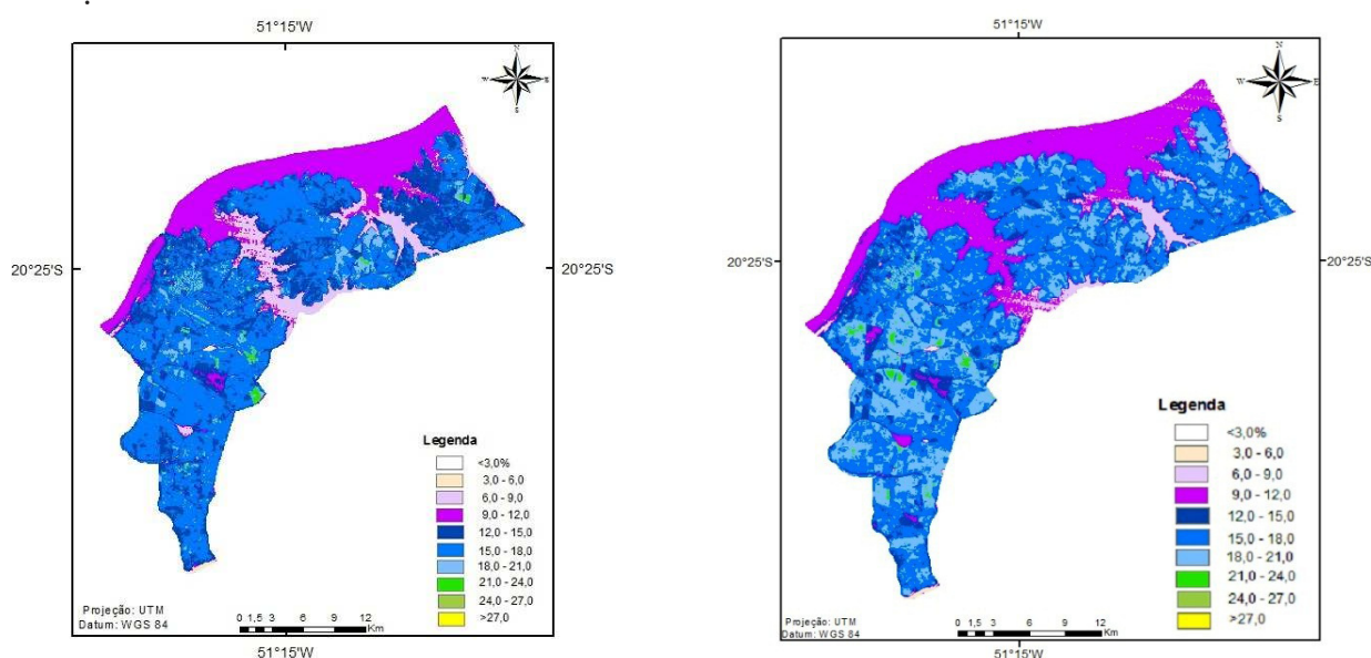
Figure 3 – Images classified of the Surface Albedo (in %), (a) for 13/May/2000 and (b) for 10/April/2011
