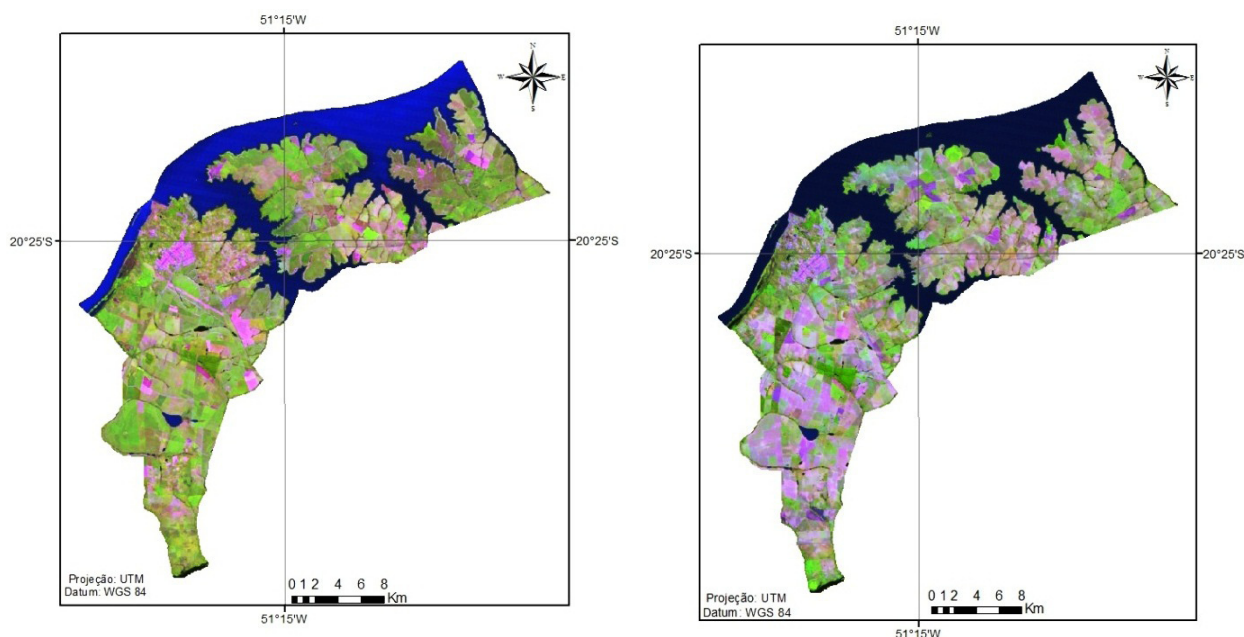
Figure 1 - Cutout of the study area in RGB composition with bands 4, 3 and 2 for (a) 13/May/2000 and (b) 10/April/2011.
