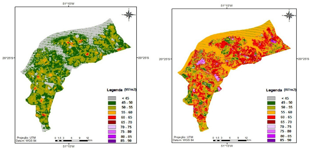
Figure 7 – Classified image of soil heat flux estimated for (a) 13/May/2000 and (b) 10/April/2011
