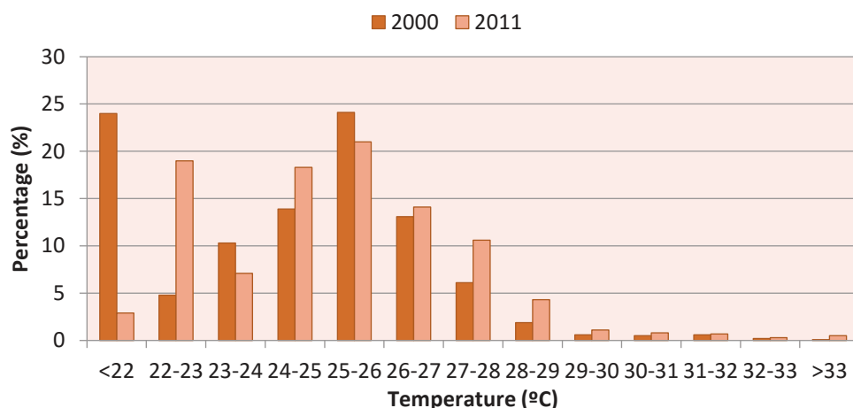
Figure 6 - Comparative histogram of surface temperature frequencies for both images used
