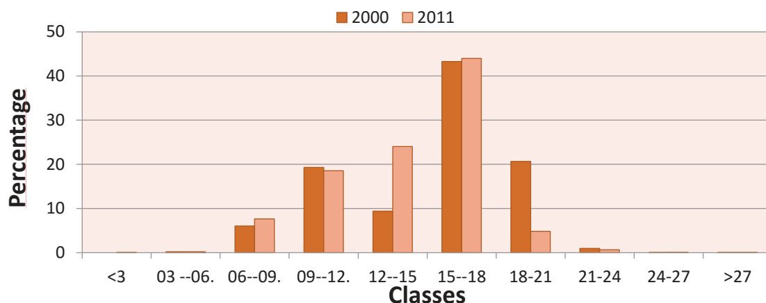
Figure 4 - Comparative histogram of Surface Albedo frequencies for the two images used
