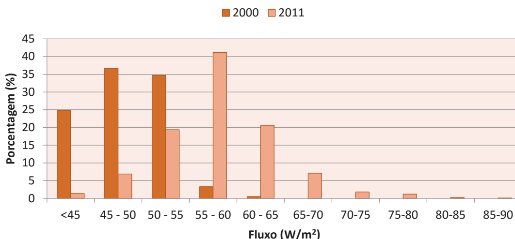
Figure 8 - Comparative histogram of soil heat flux frequencies for both images used
