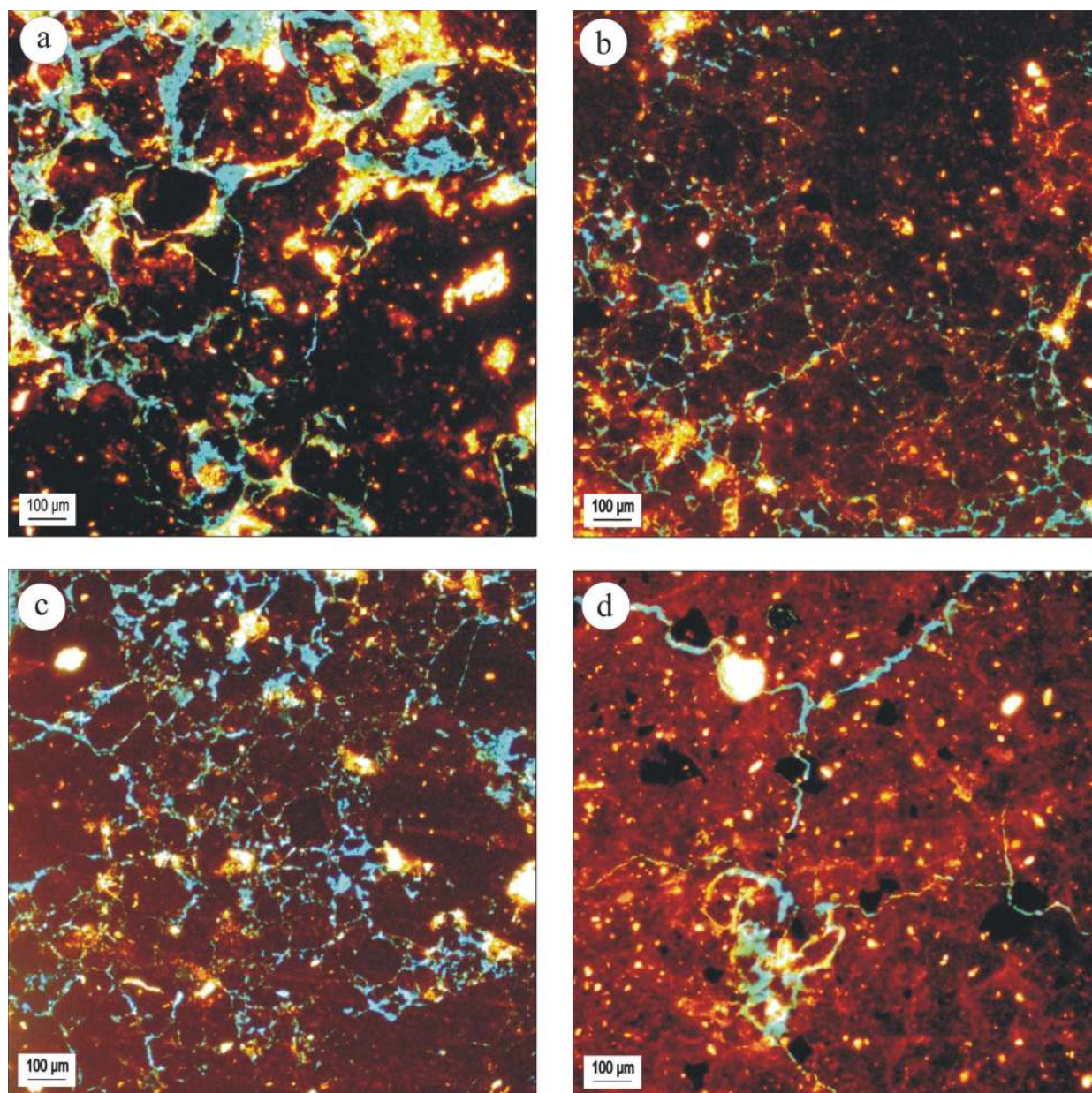
Figure 3 - Soil horizons photomicrographs from the Marechal Plateau topossequence. a) Ap volume – Transition from discontinuous porphyric fabric and enaulic fabric zone with compound packing voids. b) AB volume – Red-yellowish micromass with “stress cutans” and highlight to coalescence of microaggregates. c) Bw volume – Porphyric fabric and agglomerates of microaggregates. d) Nitic volume – Porphyric fabric, subangular polyhedral aggregates, and inter-aggregated planar dominant porosity.
