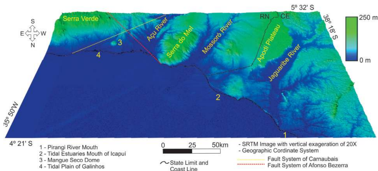
Figure 5 - Block 3D diagram of the Costa Branca (Costa do Sal) of the Brazilian Semi-arid Coast. The figure highlights the fairly low coastline between the tidal plain of Galinhos and the fluvial-marine plain of the Açu River and the great advance of the quota 0 m inside the estuary of the Mossoró River.
