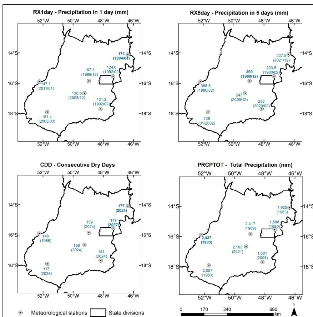
Figure 3 – Spatial variation of extreme events from from 1980 to 2024 for some indices associated with precipitation (RX1day, RX5day, CDD and PRCPTOT). Source: authors, based on INMET data processed in RCLIMDEX.
