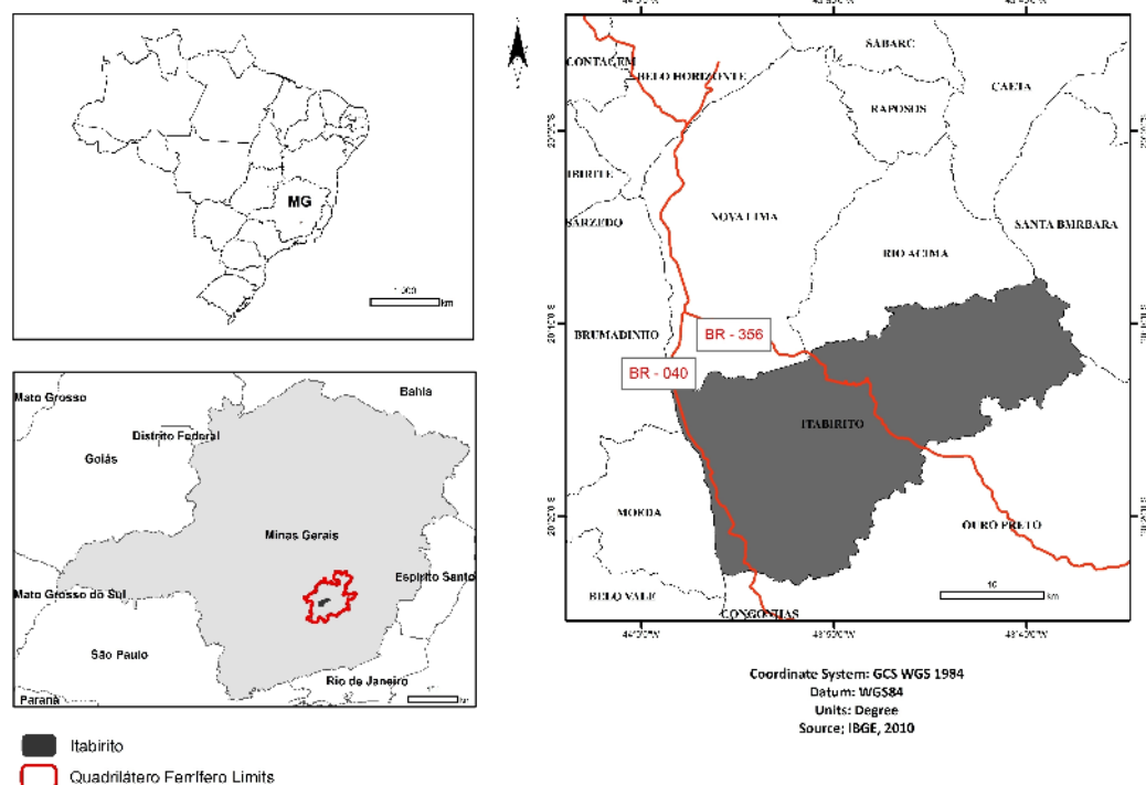
Figure 1 - Location map of the municipality of Itabirito - MG – Brazil (Source IBGE, 2010)
