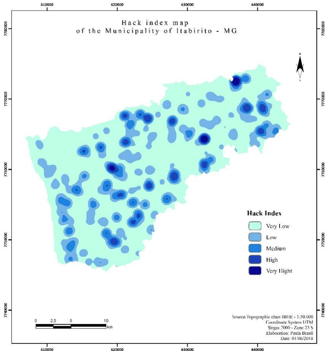
Figure 4- Hack index map of the Municipality of Itabirito
