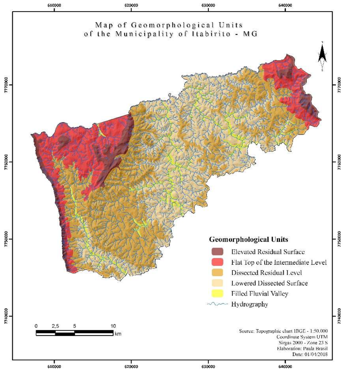
Figure 7 – Map of Geomorphological Units of the Municipality of Itabirito
