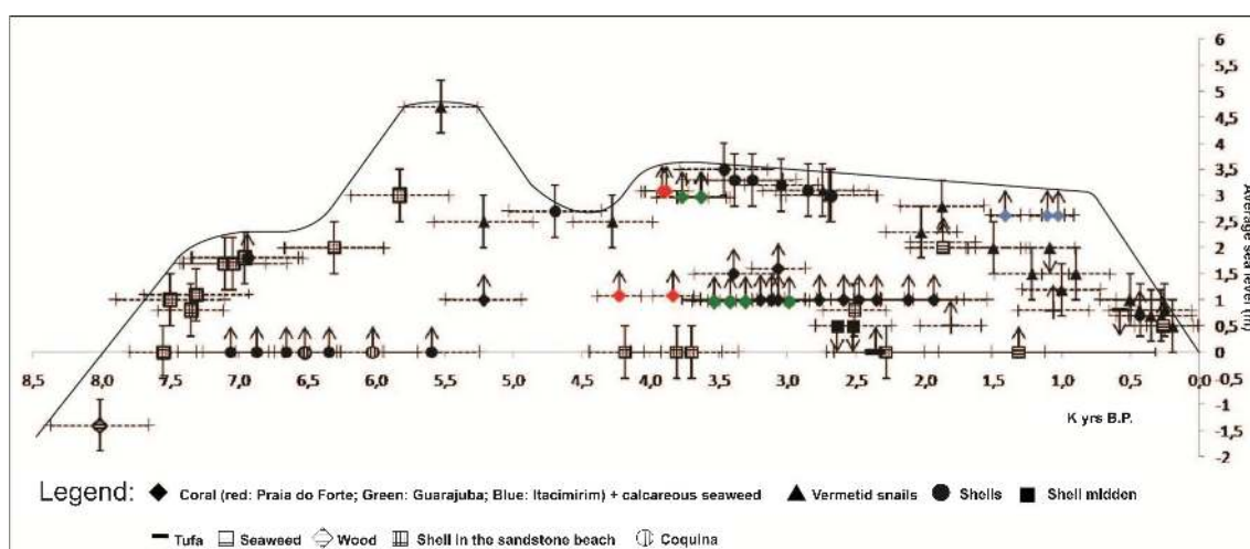
Figure 9 - Mean sea level (MSL) fluctuation curve for the last 8,000 years for the region of Salvador. Source: Gonçalves (2016, p. 27).
