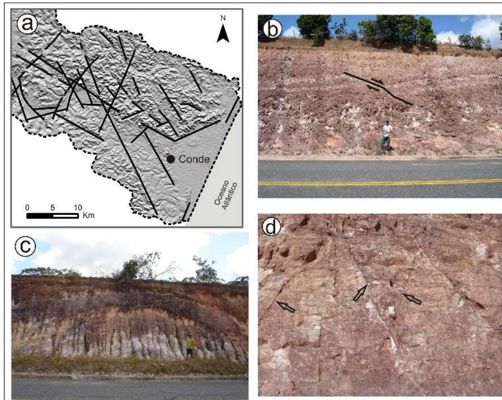
Figure 3 - Neotectonic features in the Barreiras Group sediments, near Conde: main structural lines in the low course of the Itapicuru (a); low-angle normal failure (b); anticline (c); and tectonic joints (d). Source: adapted from Dantas and Lima (2008).
