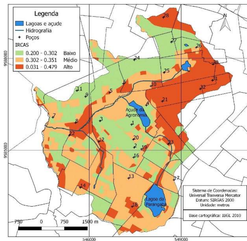
Figure 5 – The Contamination risk map
