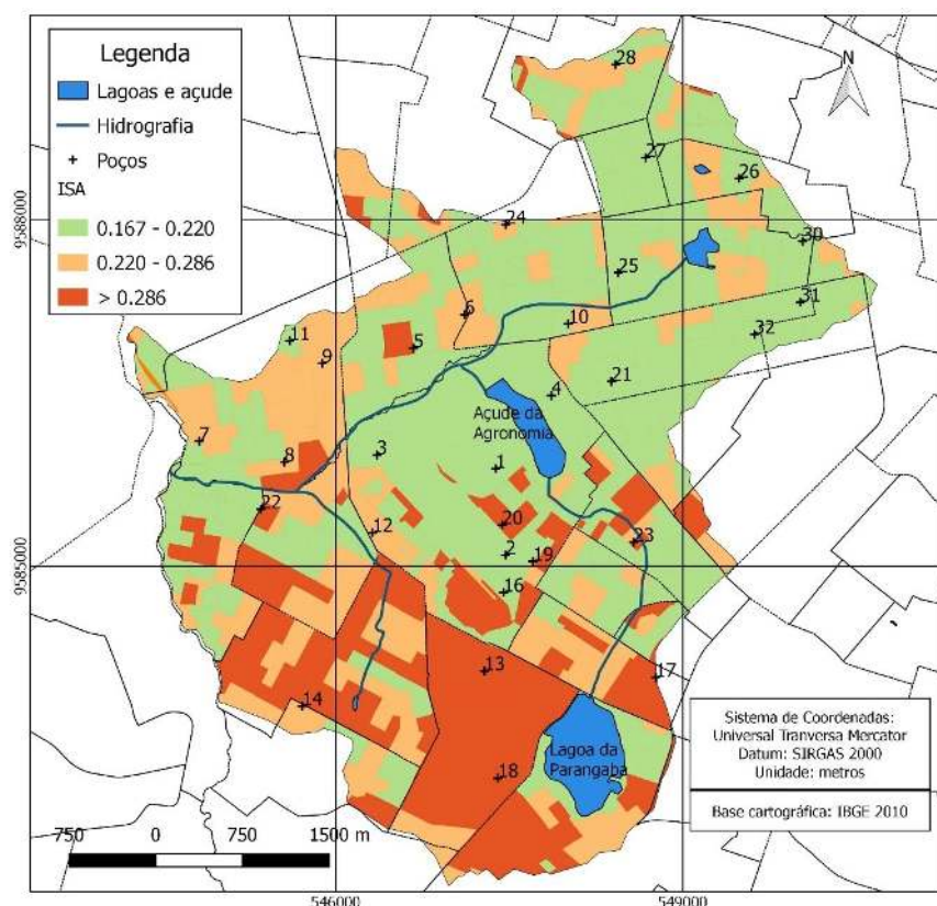
Figure 4 – The Environmental Sanitation Index Map
