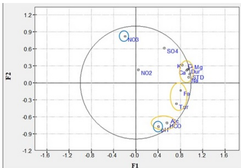
Figure 7 - ACP of well water quality in the dry period. Caption: Tur - turbidity; Fl - fluoride; Fe - iron; Alk - alkalinity; K - potassium; Ca - calcium; Mg – magnesium; Dur - hardness; Na - sodium; NO3 - nitrate; SO4 –sulfate; STD - total dissolved solids
