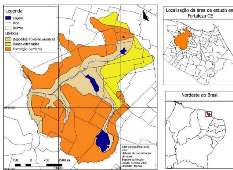
Figure 1 – The lithological units of the study area. They have the best aquifer potential, providing good flow for wells (5-5 m 3 /h) (CAVALCANTE, 1998).
