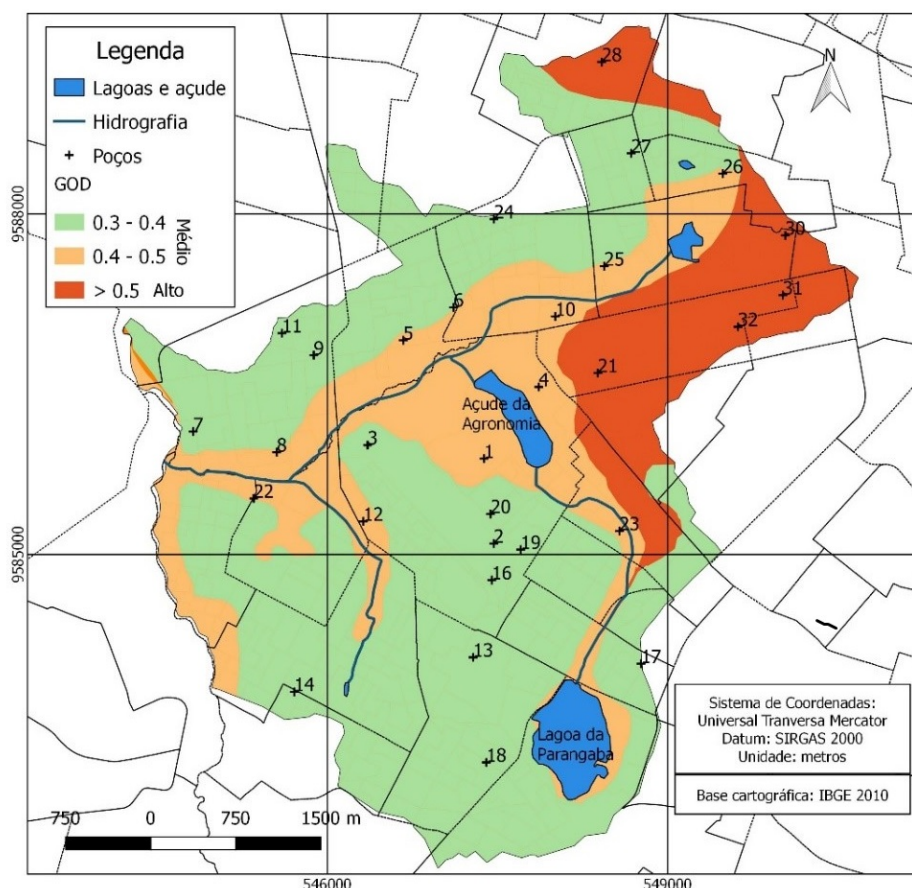
Figure 3 – The GOD aquifer vulnerability map
