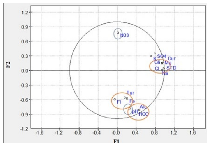
Figure 6 - ACP of well water quality in the rainy season. Caption: Tur - turbidity; Fl - fluoride; Fe - iron; Alk - alkalinity; K - potassium; Ca - calcium; Mg – magnesium; Dur - hardness; Na - sodium; NO3 - nitrate; SO4 –sulfate; STD - total dissolved solids.
