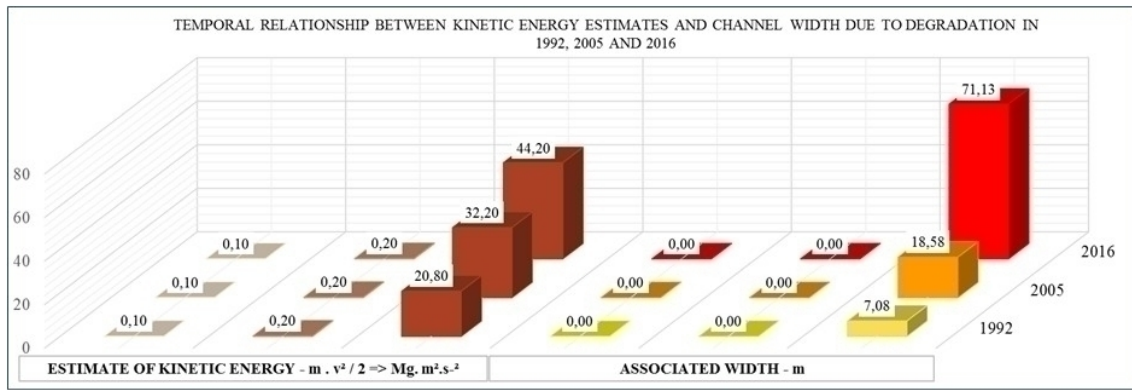
Figure 6 - Temporal relationship between the estimates of kinetic energy and the mean width of the drainage channel in the years 1992, 2005 and 2016.
