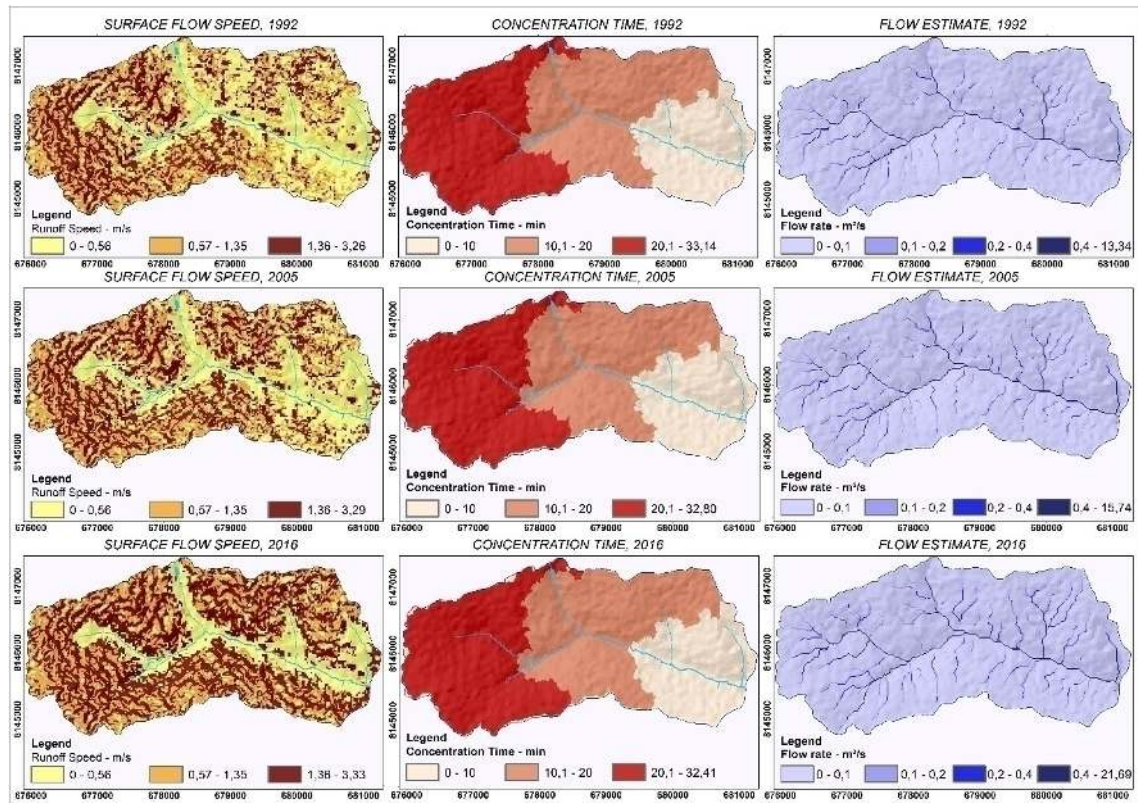
Figure 5 - Maps of velocity estimates; concentration times, and runoff volumes for 1992, 2005, and 2016.
