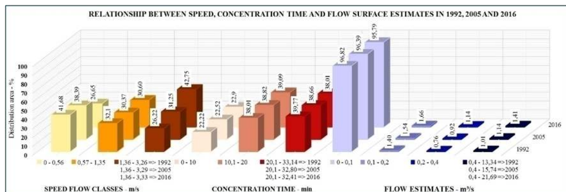
Figure 4 - Speed flow classes, concentration time, flow estimates, and respective area percentages in 1992, 2005, and 2016.
