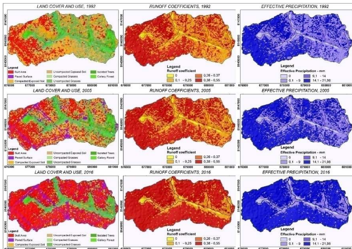
Figure 3 - Maps of land cover and use and the respective runoff and effective precipitation coefficients in 1992, 2005, and 2016.
