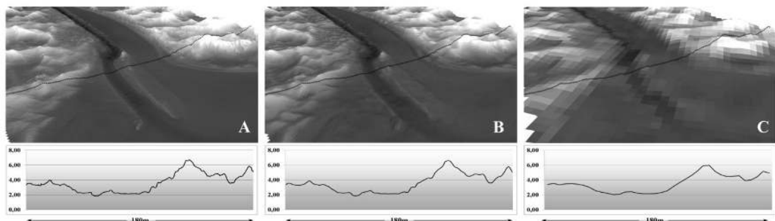
Figure 3 - Examples of the DEMs of a depositional coastal plain at different spatial resolutions. A) The centimeter resolution (GSD 0.05 m) results in a topographic profile with the greatest detail of the terrain inflections; B) By decreasing the resolution (GSD 1.0 m) the topographic profile presents a major degree of smoothing; C) The topographic profile generated using a much a coarser resolution (GSD 5.0 m) presents a high degree of homogeneity in the forms.
