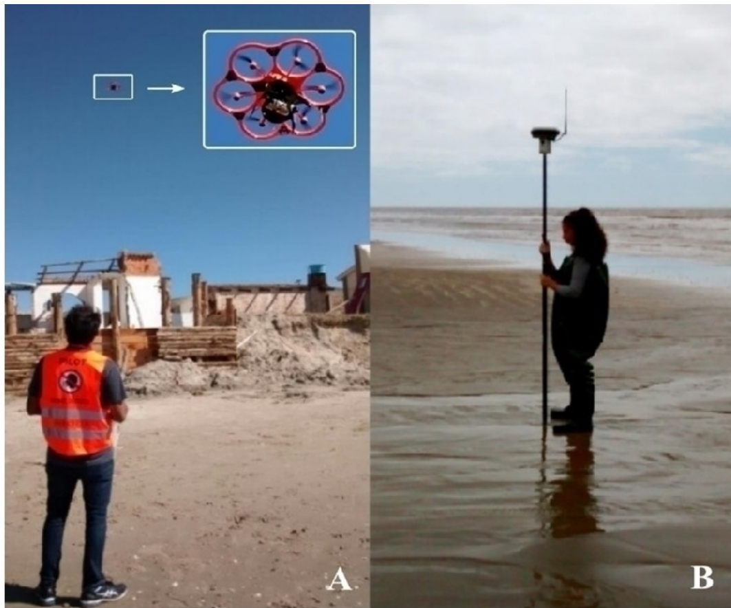
Figure 5 - Different approaches for the collection of coastal data. A) Aerophotogrammetric survey using a UAV; B) Geodetic survey using GNSS equipment.
