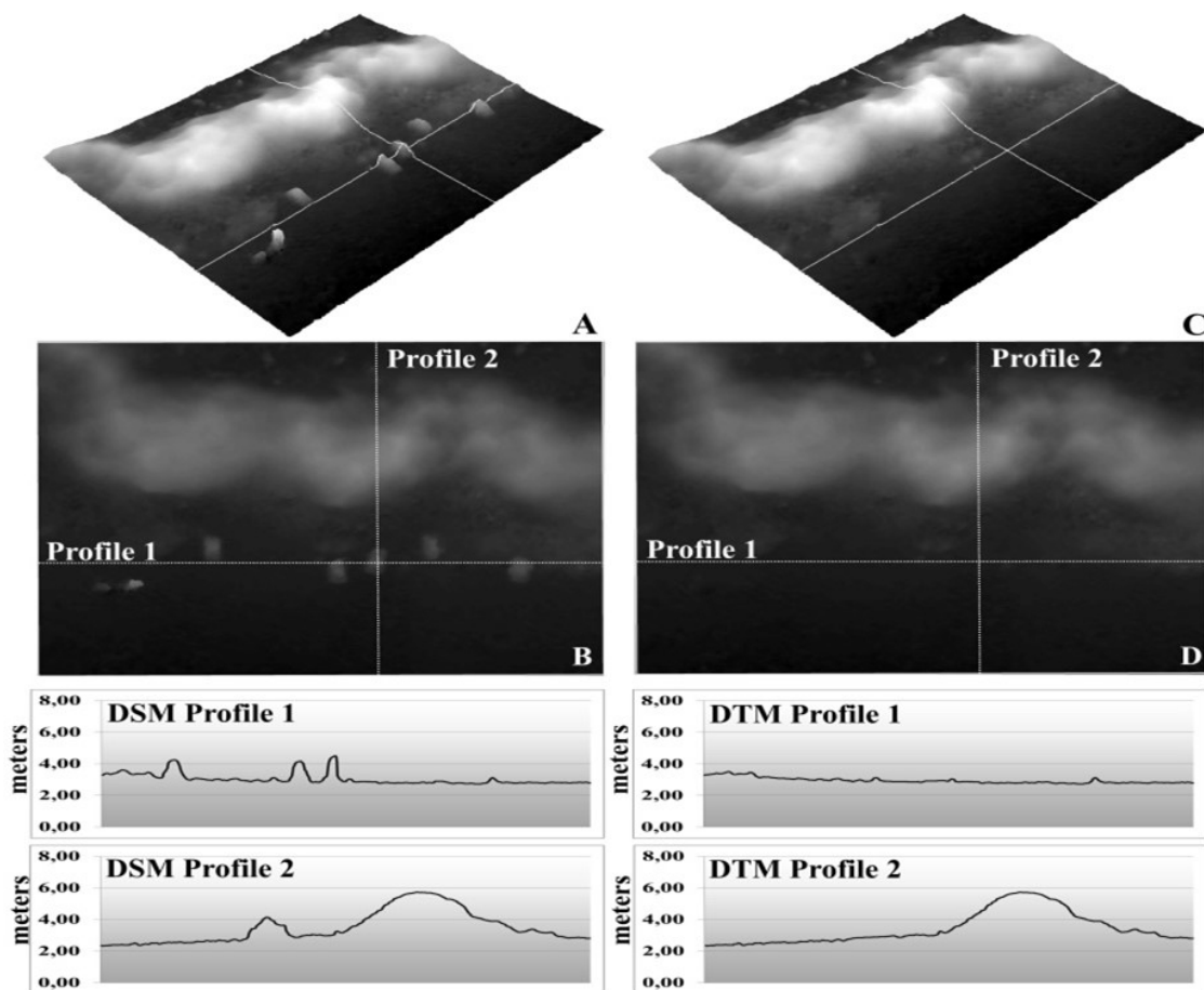
Figure 8 - Profiles showing the geomorphometric difference between DSMs and DTMs. A and B) The topo-graphic transition between beach and dune - profiles 1 and 2 highlight the presence of artifacts, that is, cars parked at the seafront (DSM); C and D) The same study area, but with the artifacts omitted by the dense cloud classification method (DTM).
