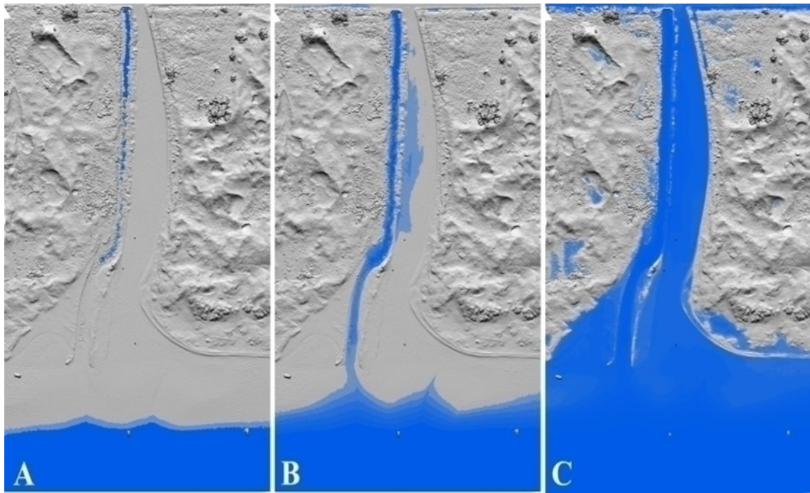
Figure 6 - Example of a simple bathtub model obtained using GIS software for different SLR values applied to a coastal DEM. A) 10 centimeter SLR simulation; B) 50 centimeter SLR simulation; C) 1 meter SLR simulation.
