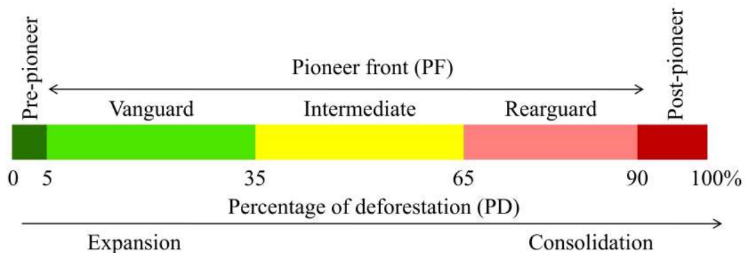
Figure 3 - Cartographic model of the pioneer fronts in the Brazilian state of Pará (adapted from Thalês; Poccard-Chapuis, 2014).
