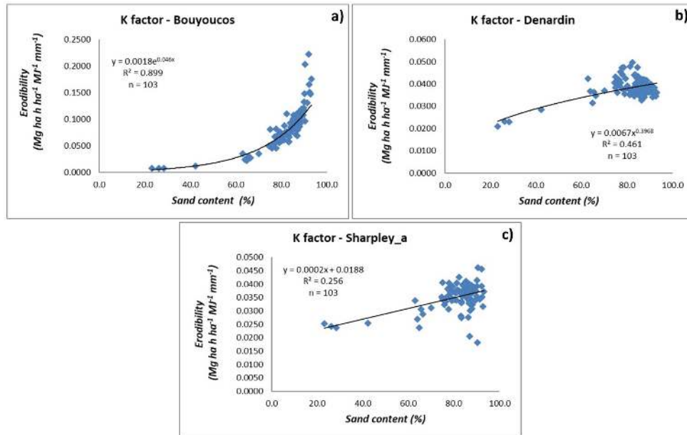
Figure 3 - Trend lines between the main (positive) interactions of erodibility with the sand content of PRHB soils.
