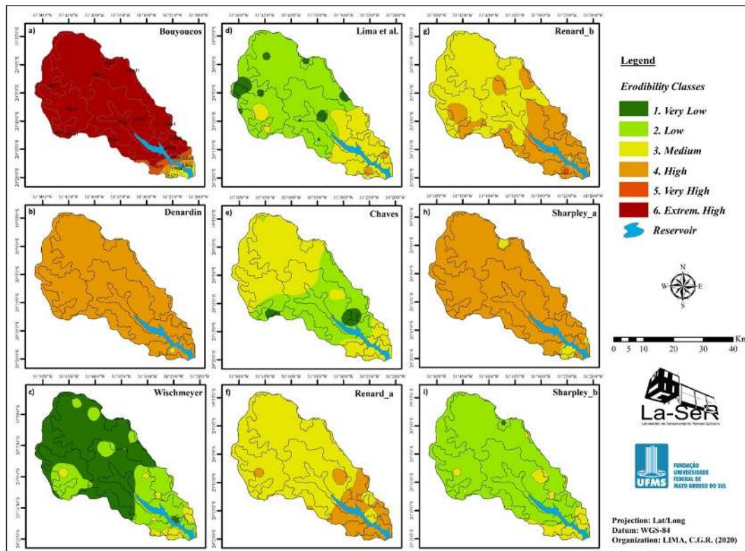
Figure 5 - Kriging maps of soil erodibility in the PRHB for different determination methodologies.
