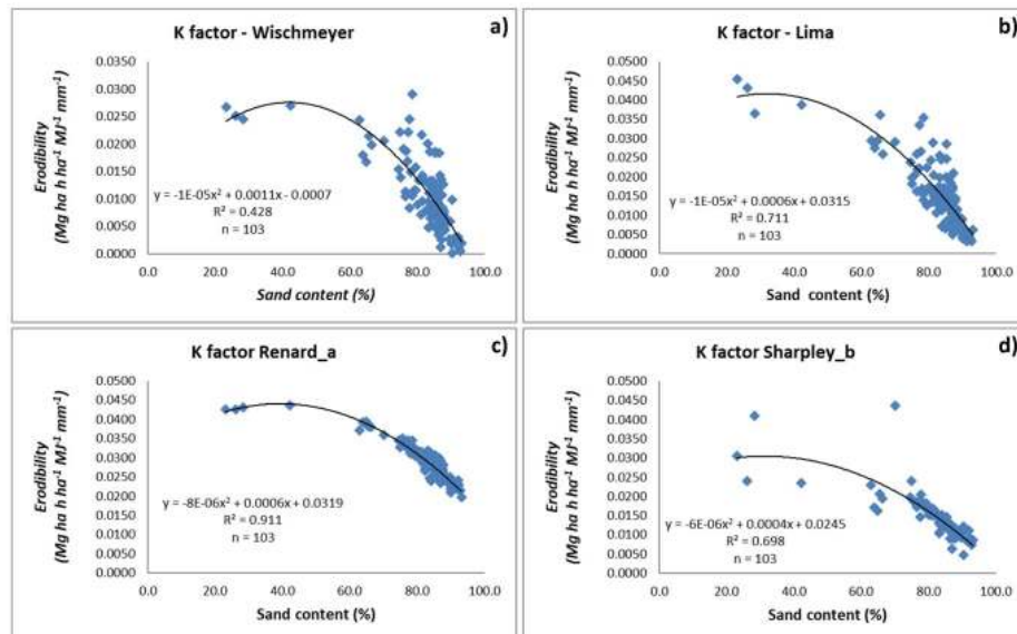
Figure 4 - Trend line between the main (negative) interactions of erodibility with the sand content of PRHB soils.
