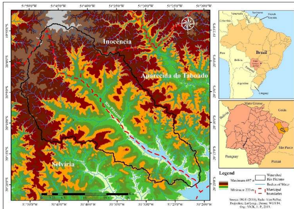
Figure 1 - Location of the study area, PRHB.
