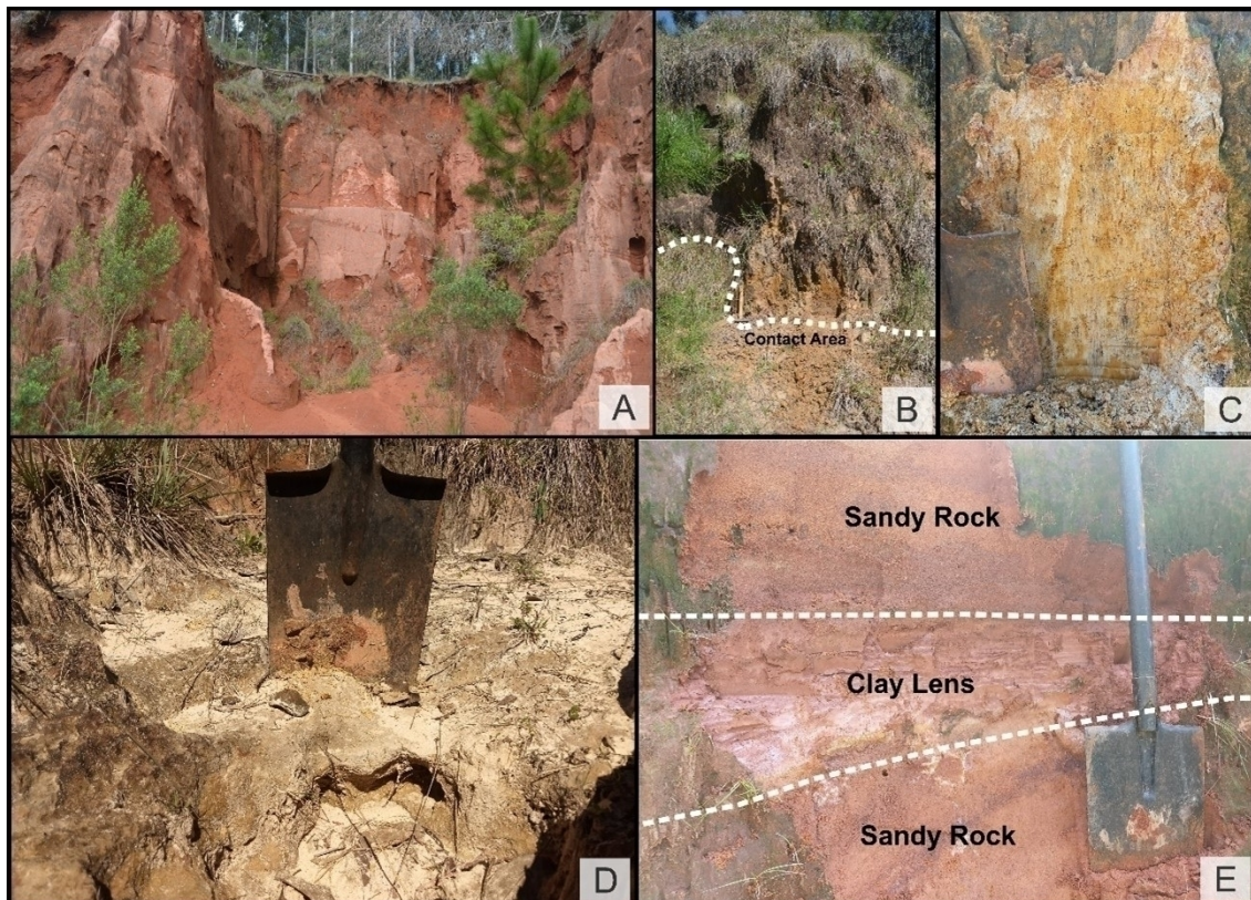
Figure 11 - A - Occurrence of mass movement in sector B of Areal Gully; B - Contact area of the sandiest rock portion with the most clayey portion; C - Mottled aspect of altered clayey rock blade; D - Sandy portion of the slope with loss of color; E – Alternation of rock lenses with different characteristics in Areal Gully.
