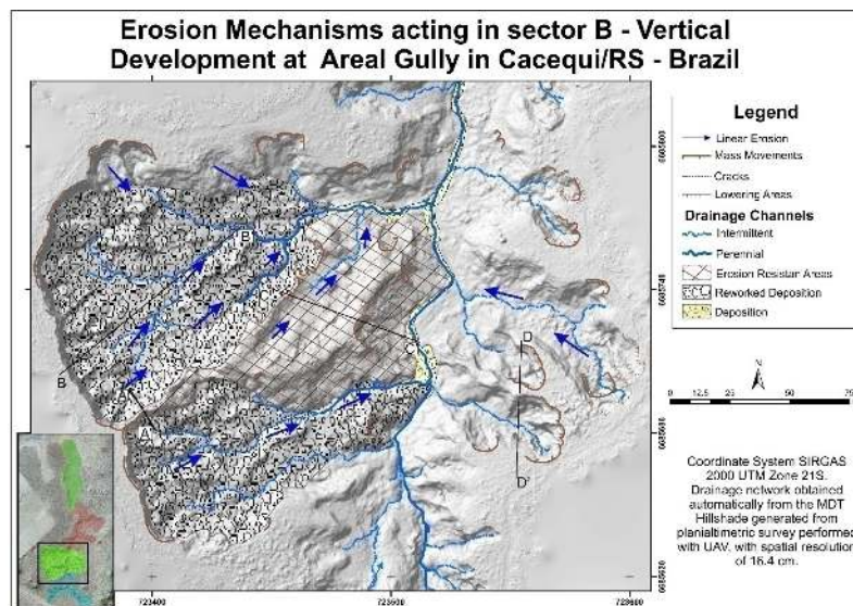
Figure 5 - Map of erosive mechanisms operating in sector B of Areal Gully.
