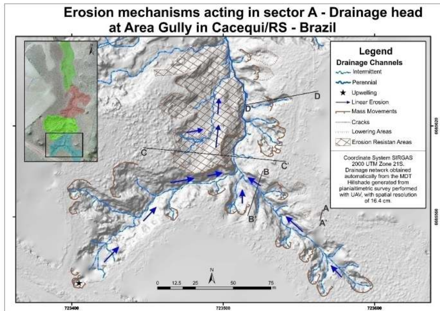
Figure 3 - Map of erosive mechanisms operating in sector A of Areal Gully.
