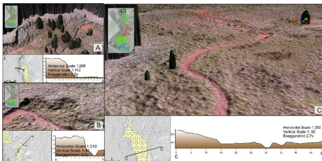
Figure 10 - Schematic representation of the erosive mechanisms acting in sector D (A - Mass movements; B- Small mass movements and associated cracks; C - Flat area).
