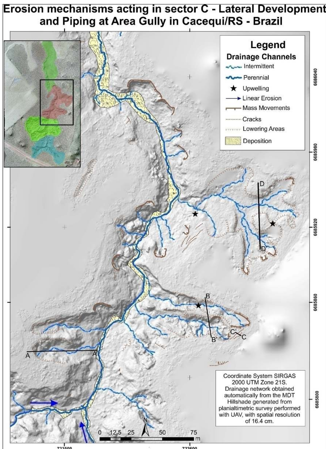
Figure 7 - Map of erosive mechanisms operating in sector C of Areal Gully.
