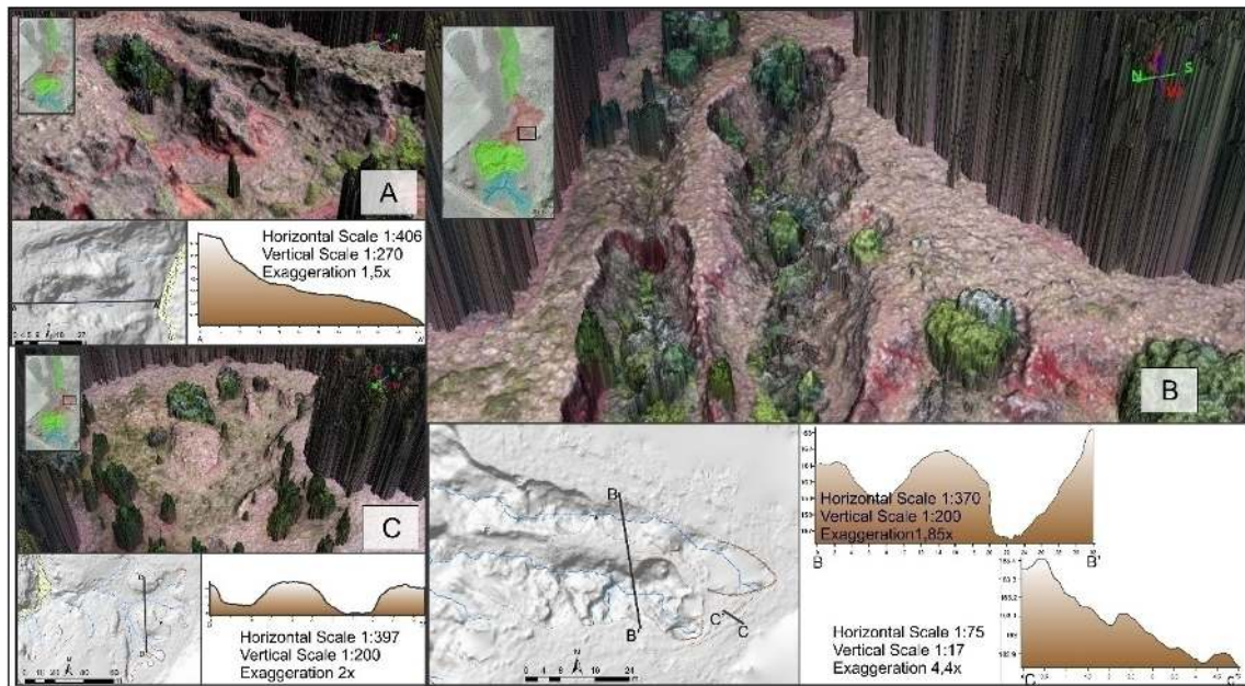
Figure 8 - Schematic representation of the mechanisms acting in sector C (A - Downgrade area; B - Parallel branches associated with the downgrade and crack formation areas; C - Downgrade area).
