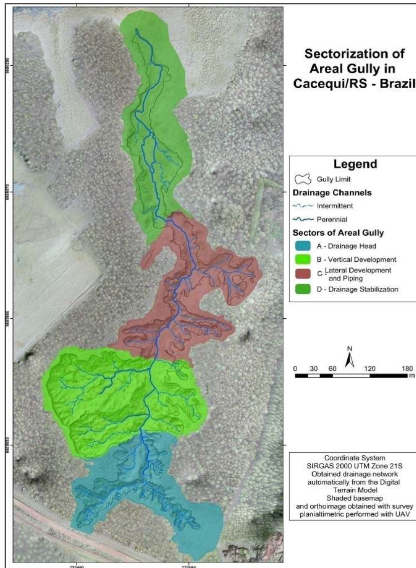
Figure 2 - Sectors of Areal Gully in Southern Brazil.
