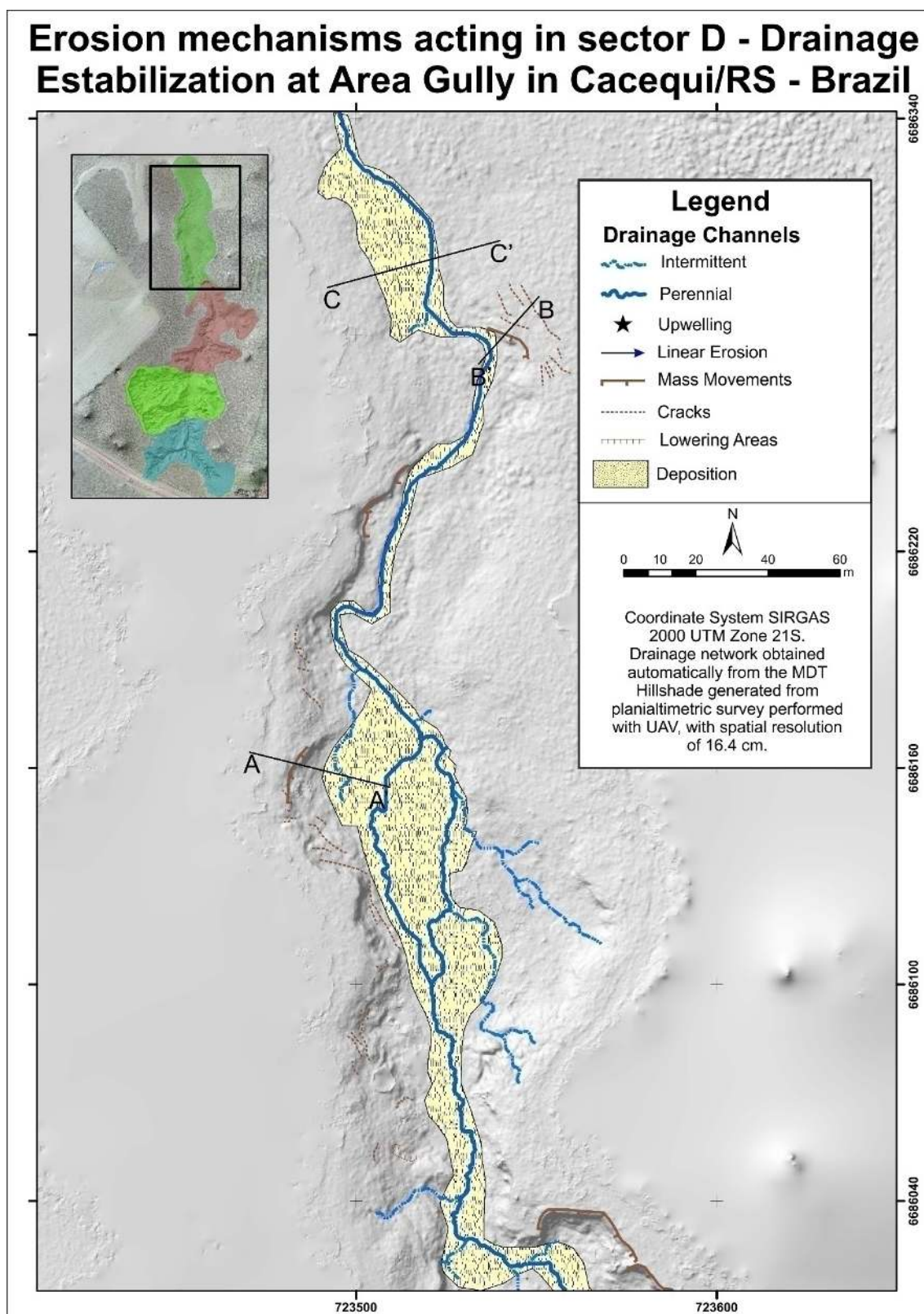
Figure 9 - Map of erosive mechanisms operating in sector D of Areal Gully.
