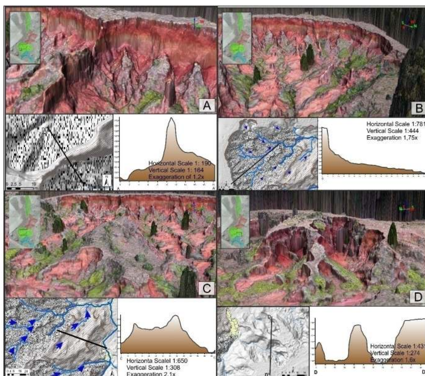
Figure 6 - Schematic representation of the mechanisms acting in sector B (A - Erosion resistant line; B - Vertical development area; C - Erosion resistant area; D - Area of occurrence of intense mass movements).
