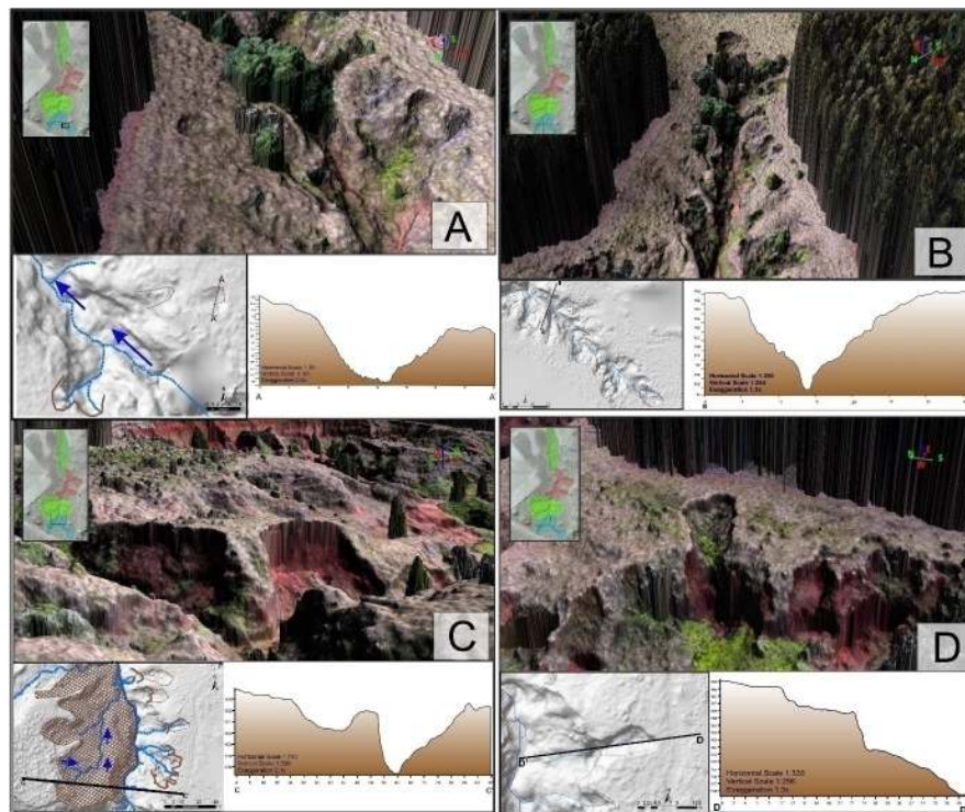
Figure 4 - Schematic representation of the mechanisms acting in sector A (A - Lowering Area; B - Linear Erosion; C - Erosion-resistant portion; D - Lowering followed by mass movement).
