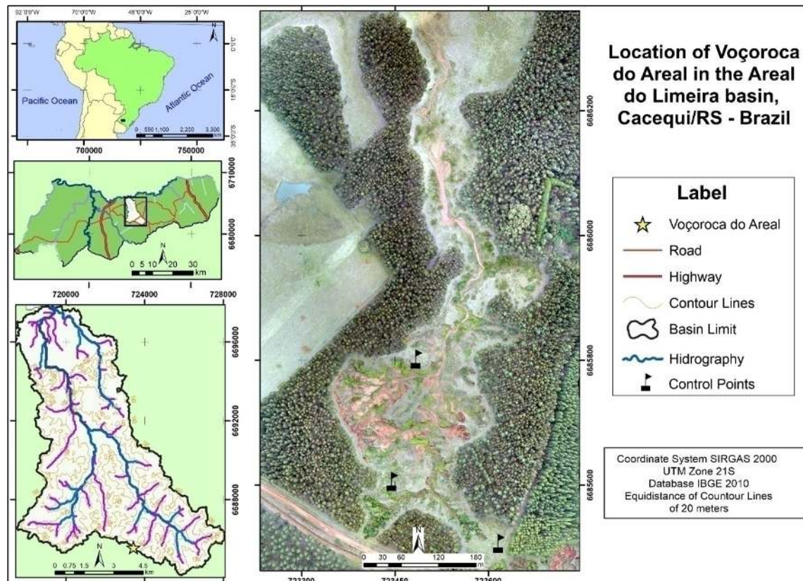
Figure 1 - Localization of Areal Gully
