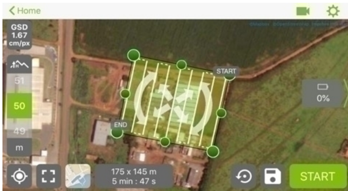
Figure 1 - Flight plan of the area of interest to be mapped in Goianópolis, programmed in the Pix4D Capture software, with the flight lines adjusted according to the lateral and longitudinal overlap suitable for this project (60 x 70%) at a flight height of 50 m.
