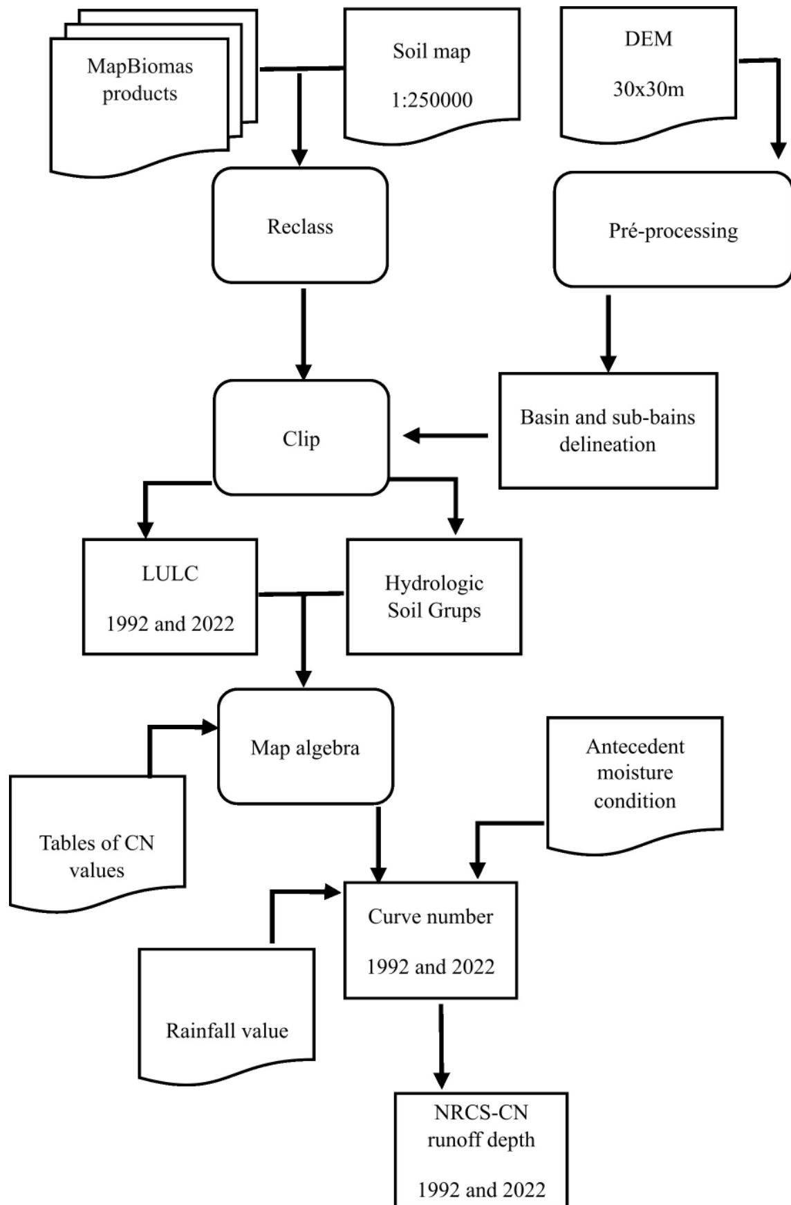
Figure 2 - Flowchart with the methodology for determining surface runoff through the NRCS-CN method in a GIS environment
