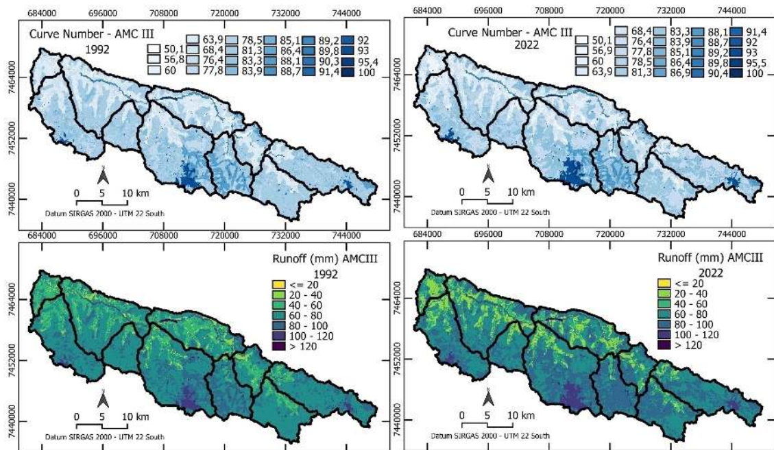
Figure 9 - Curve Number values and surface runoff depth, considering the antecedent runoff condition III and a rainfall of 130 mm for 1992 and 2022.
