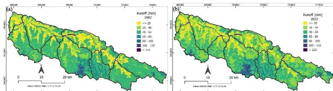
Figure 8 - Surface runoff depth considering a rainfall of 130 mm (a) in 1992, (b) in 2022.
