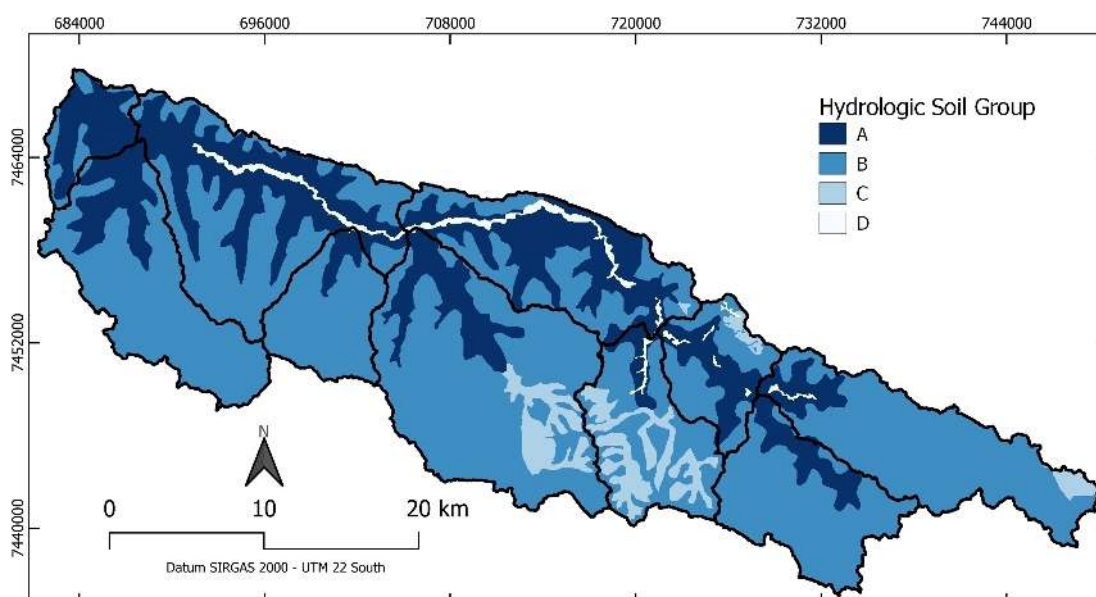
Figure 5 - Hydrologic Soil Groups
