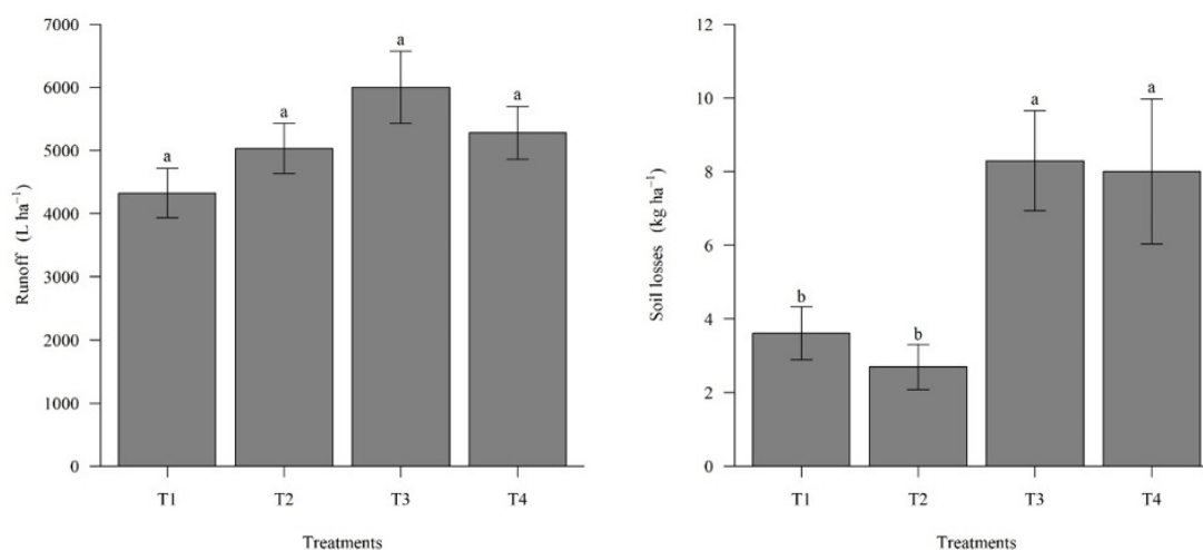
Figure 5 – Surface runoff and soil losses from treatments T1 - Planting on Contour Lines associated with stone cords + grass planting; T2 - Planting down the hill, absent of grass; T3 - Planting on a contour line + planting grass and T4 - Planting downhill + planting grass. Source: Elaboration: the authors, 2024.
