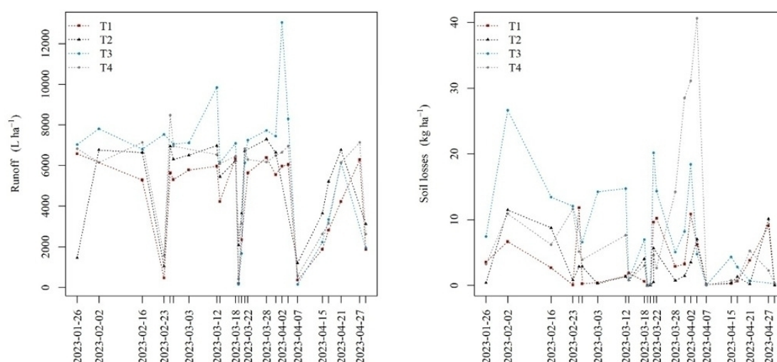
Figure 6 – Behavior of surface runoff and soil losses throughout the evaluations in the treatments T1 - Planting on Contour Lines associated with stone cords + grass planting; T2 - Planting down the hill, absent of grass; T3 - Planting on a contour line + planting grass and T4 - Planting downhill + planting grass. Source: Elaboration: the authors, 2024.
