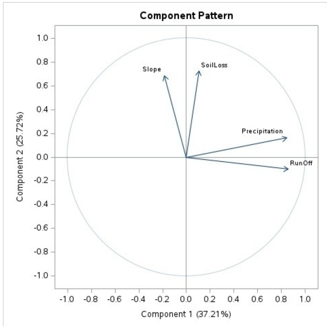
Figure 7 – Principal component analysis (PCA) for the variables precipitation, slope, soil loss and surface runoff in relation to the treatments T1 - Planting on contour lines associated with stone cords + grass planting; T2 - Planting down the hill, absent of grass; T3 - Planting on a contour line + planting grass and T4 - Planting downhill + planting grass. KMO test: 0.659 and Bartlett test: 103.776. Source: Elaboration: the authors, 2024.
