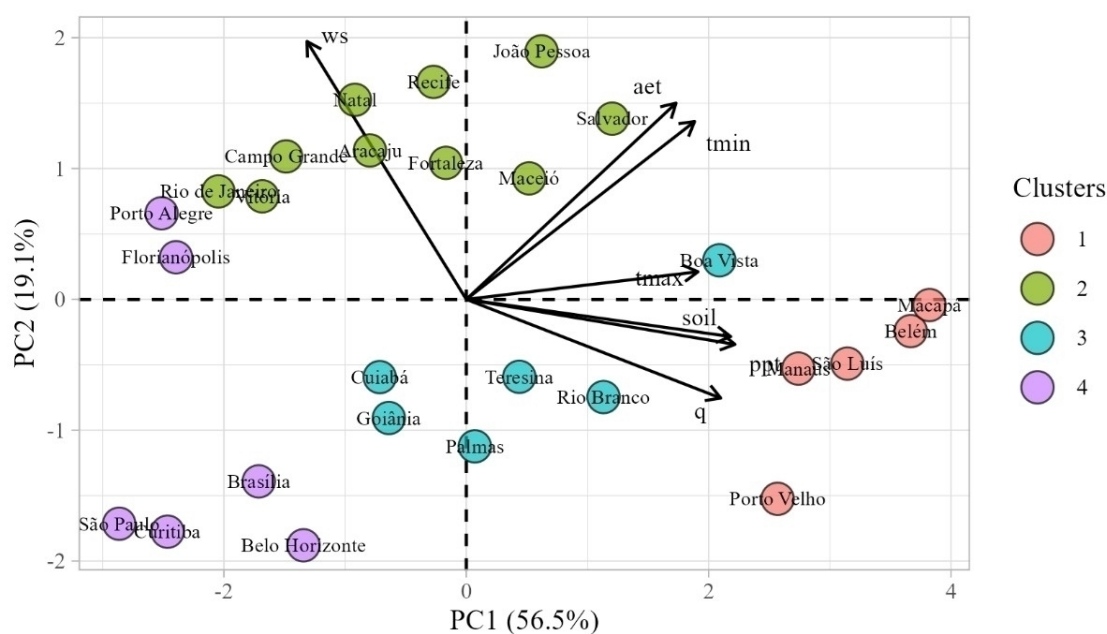
Figure 5 – Biplot with identification of the clusters on the annual averages of the variables maximum temperature ( t_{max} ), minimum temperature ( t_{min} ), precipitation ( ppt ), wind speed ( ws ), runoff ( q ), evapotranspiration ( aet ) and soil moisture ( soil ), referring to the 27 Brazilian capitals for the period from 1958 to 2022.
