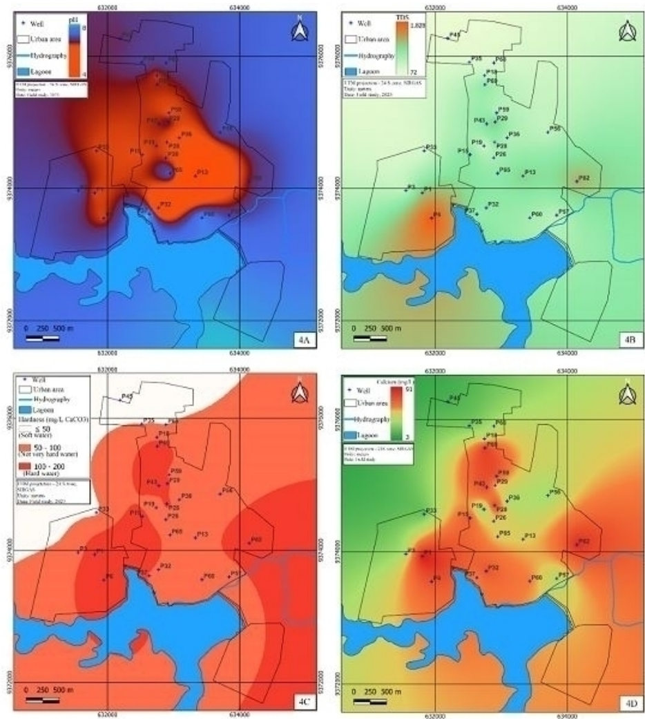
Figure 4 – Zoning of parameters: (A) Zoning of pH; (B) Zoning of TDS; (C) Zoning of Hardness; (D) Zoning of Ca +
